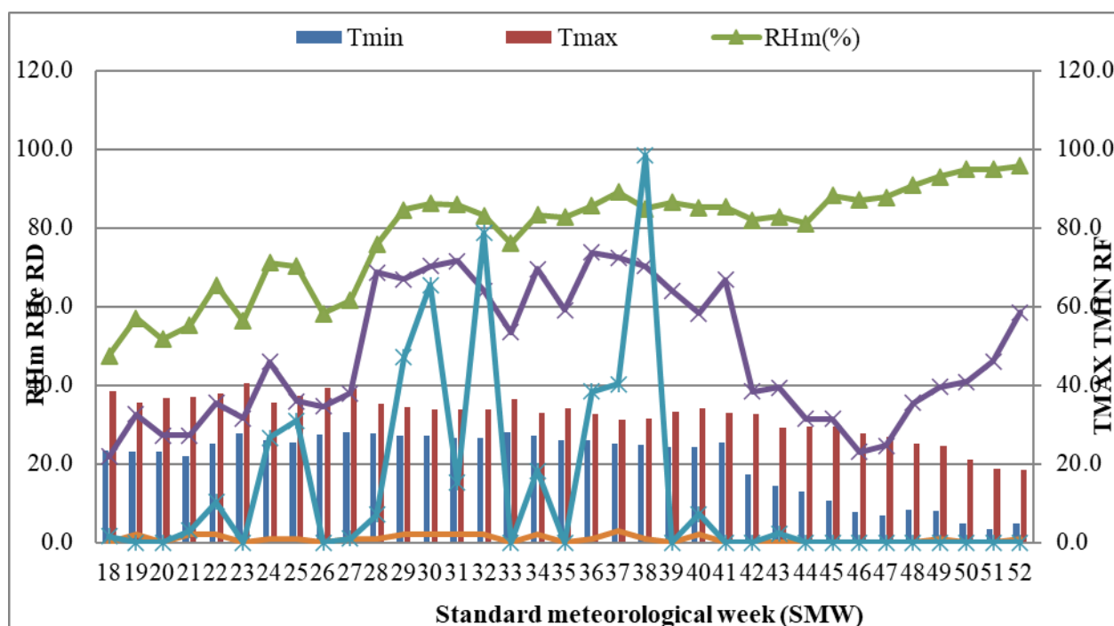
Figure 2. Weather conditions at Faridkot during kharif season 2021-22
