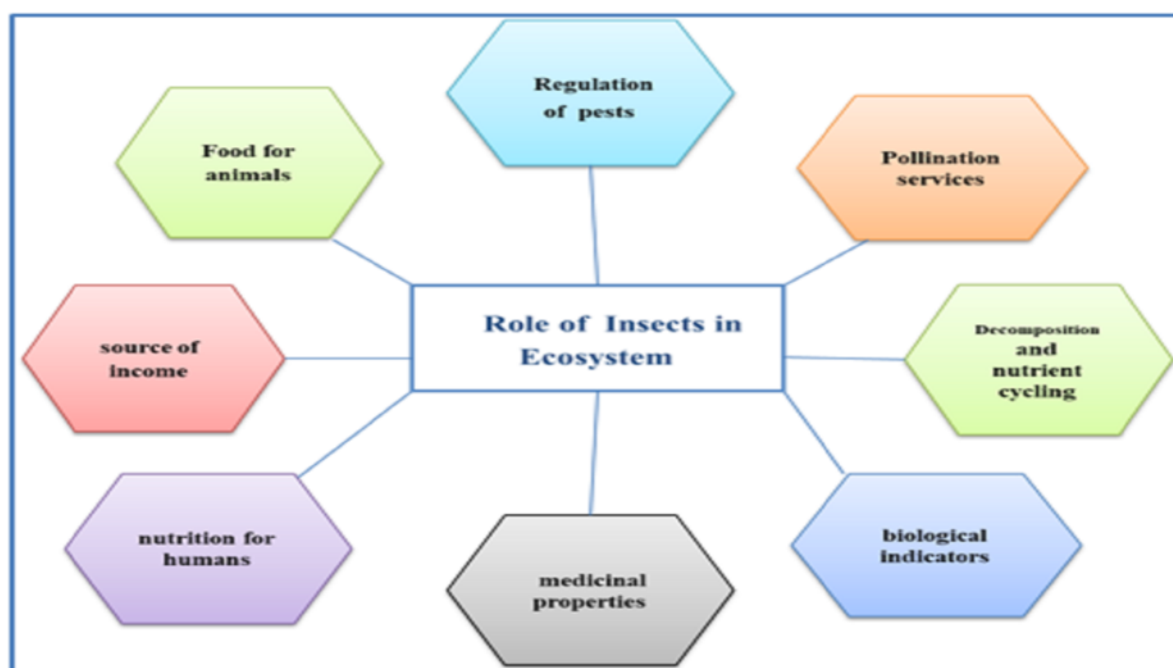
Figure 1. The Role of Insects in Ecosystem (Source: Mansowr ZF, 2025)
