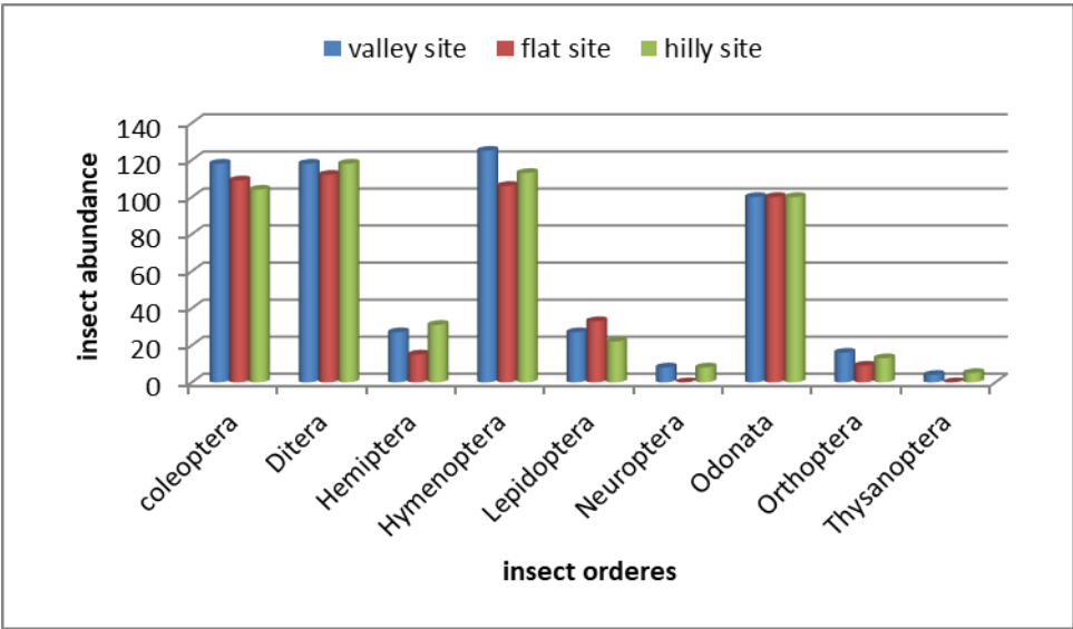
Figure 5. Insect abundance based on the total counts of sampled orders from the three elevated sites
